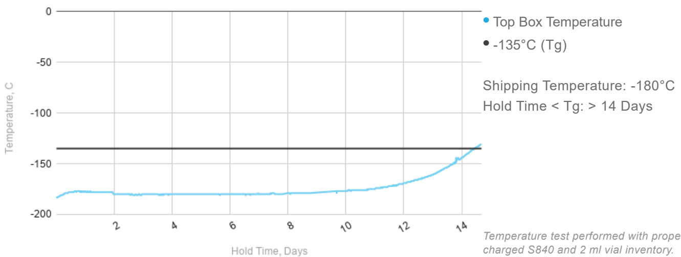
S840 Temperature Test
